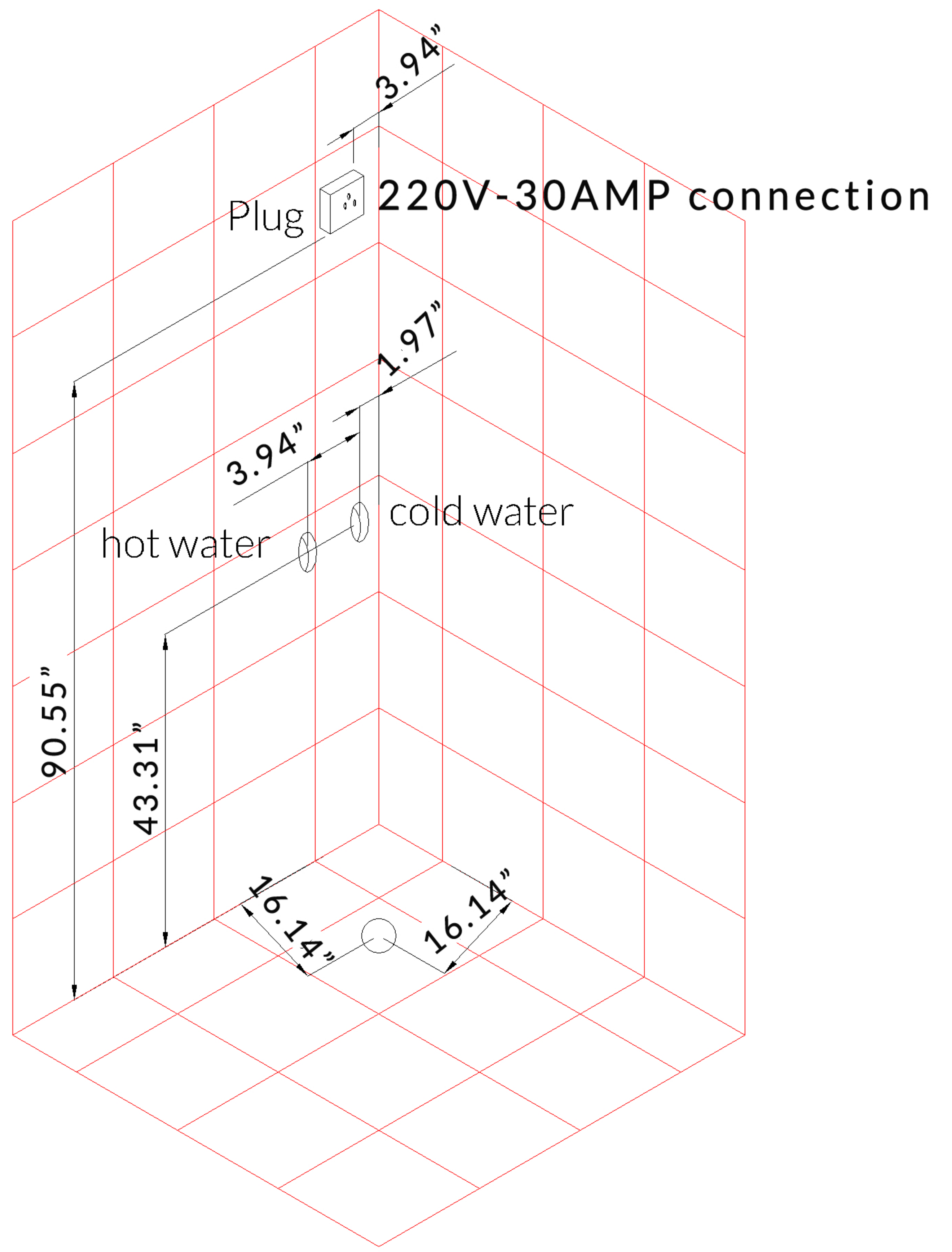
DZ961-1F8 INSTALLATION (LEFT) DIMENSIONS: 59" x 35" x 89"
